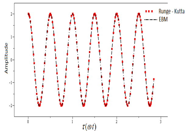
Fig. 2 Variation of the nondimensional amplitude ratio versus \tau for W_{max} = 1 and W_{max} = 2
