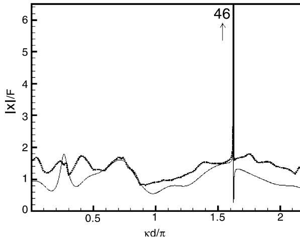
Fig. 5. Horizontal force on cylinder 1 of the circular array (Fig. 1) and (thick dotted line) on cylinder 3 of the large array (Fig. 2).
