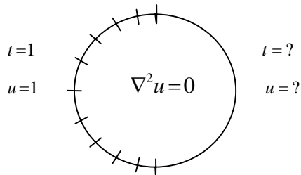
ill-posed problem
