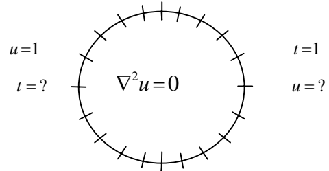
well-posed problem
