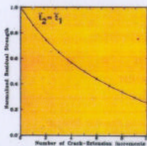
Residual strength diagram
