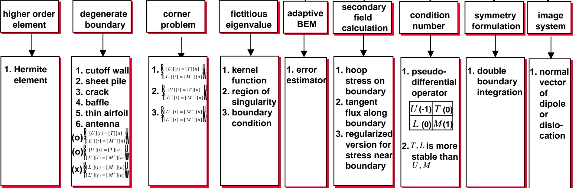
Fig.1.4 Roles of hypersingularity of boundary element method
