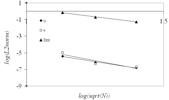
Figure 13 The convergence rate of the infinite plate with a circular hole. a) H^1 error norm and b) L^2 error norm of displacements and normal stress
