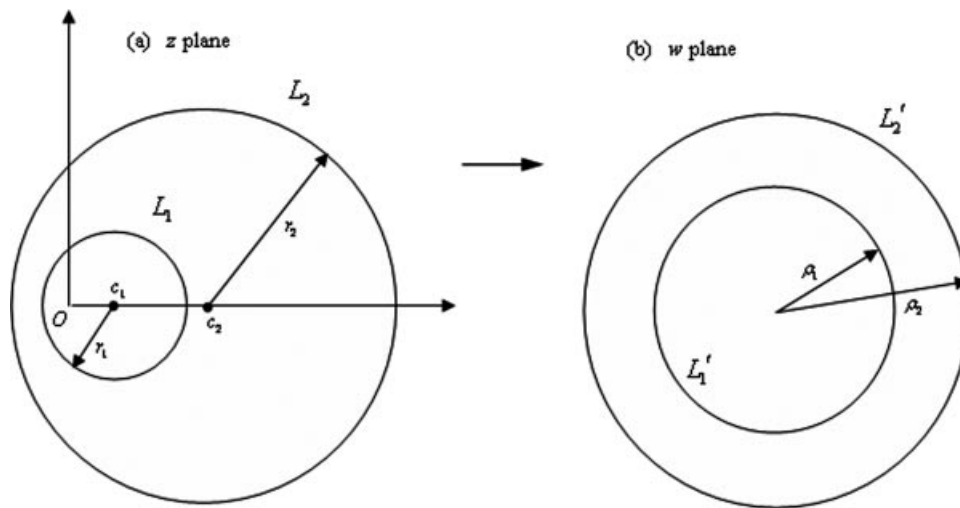
Figure 1 Mapping of w(z) = \frac{z+1}{z+4} from the eccentric region to a concentric region.
