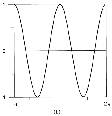
(b) Spurious boundary mode t(\theta)=\cos \theta for the Dirichlet problem.
