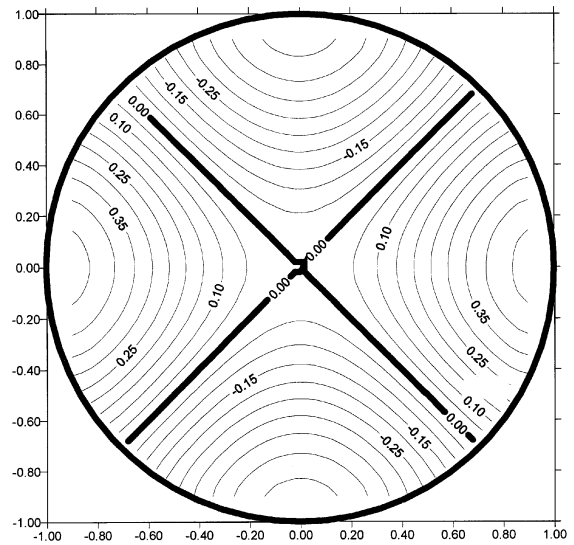
(a) Spurious interior mode u_2(a, \phi) = J_1(3.0542a)\cos 2\phi
