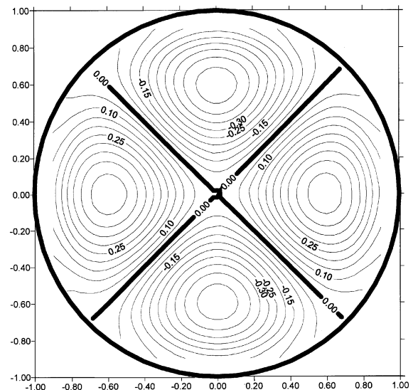
(b) True interior mode u_2(a, \phi) = J_2(5.1356a)\cos 2\phi
