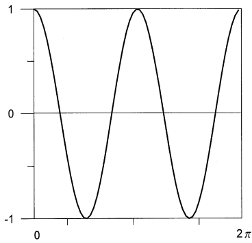
(a) True boundary mode t(\theta)=\cos 2\theta for the Dirichlet problem.
