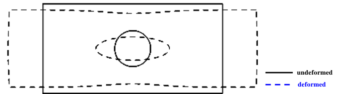
Fig. 4(c) Deformation of an infinite plate with a circular hole subject to remote tension
