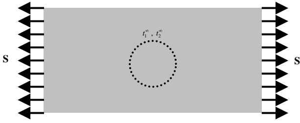
Fig. 3(a) An infinite plate subject to a uniform tension
