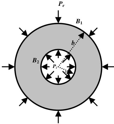
Fig. 2 An annular cylinder subject to uniform pressures
