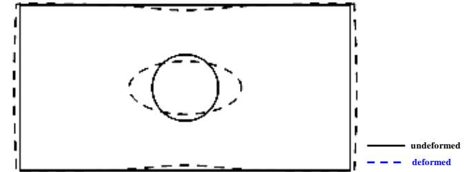
Fig. 4(b) Deformation of an infinite plate with a hole
