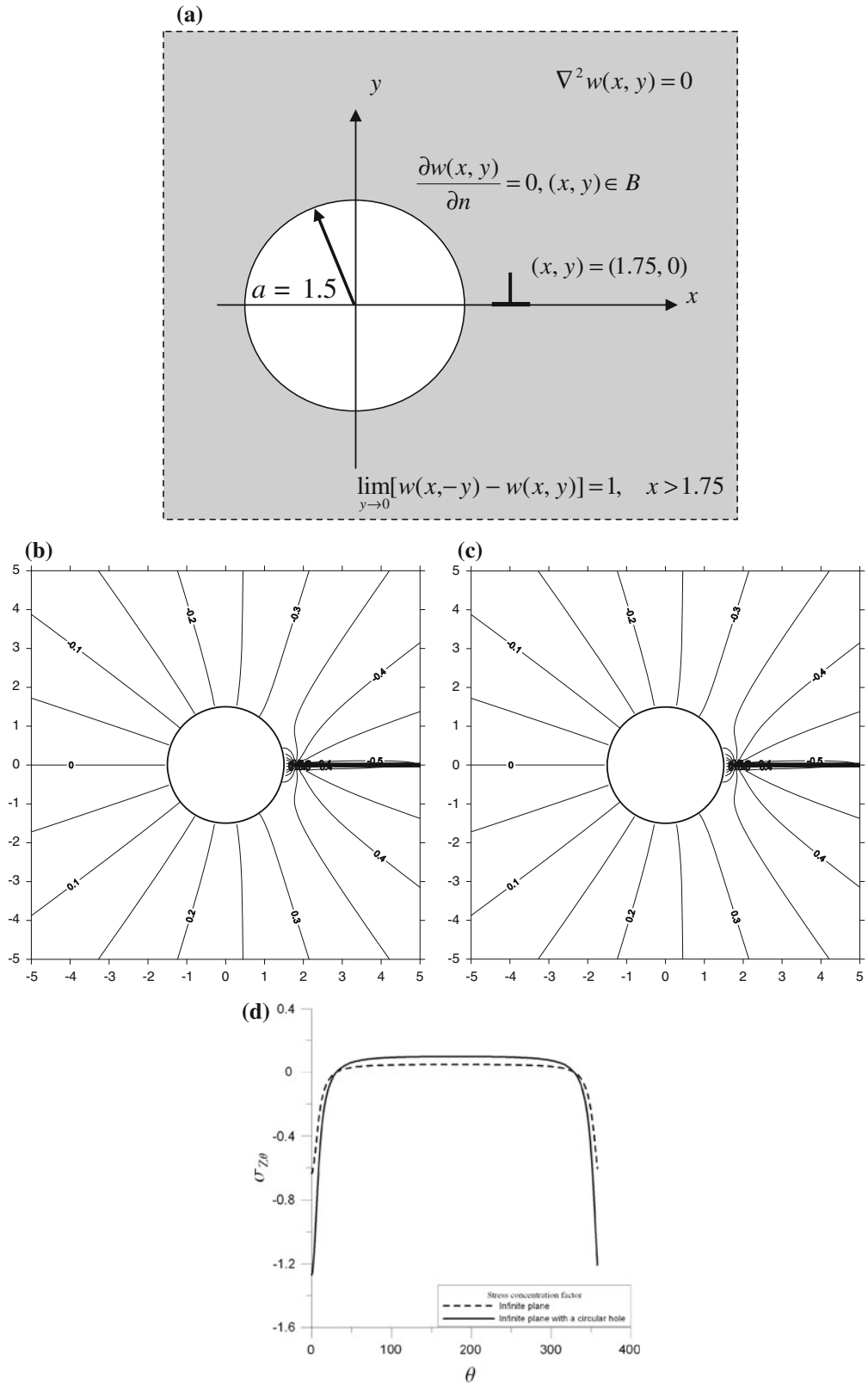
Fig. 9 a An infinite plane with a circular hole (Neumann boundary condition) subject to the screw dislocation; b Potential contour by using the Smith method [15]; c Potential contour by using the present method ( M = 50 ); d Stress distribution along the circular hole
