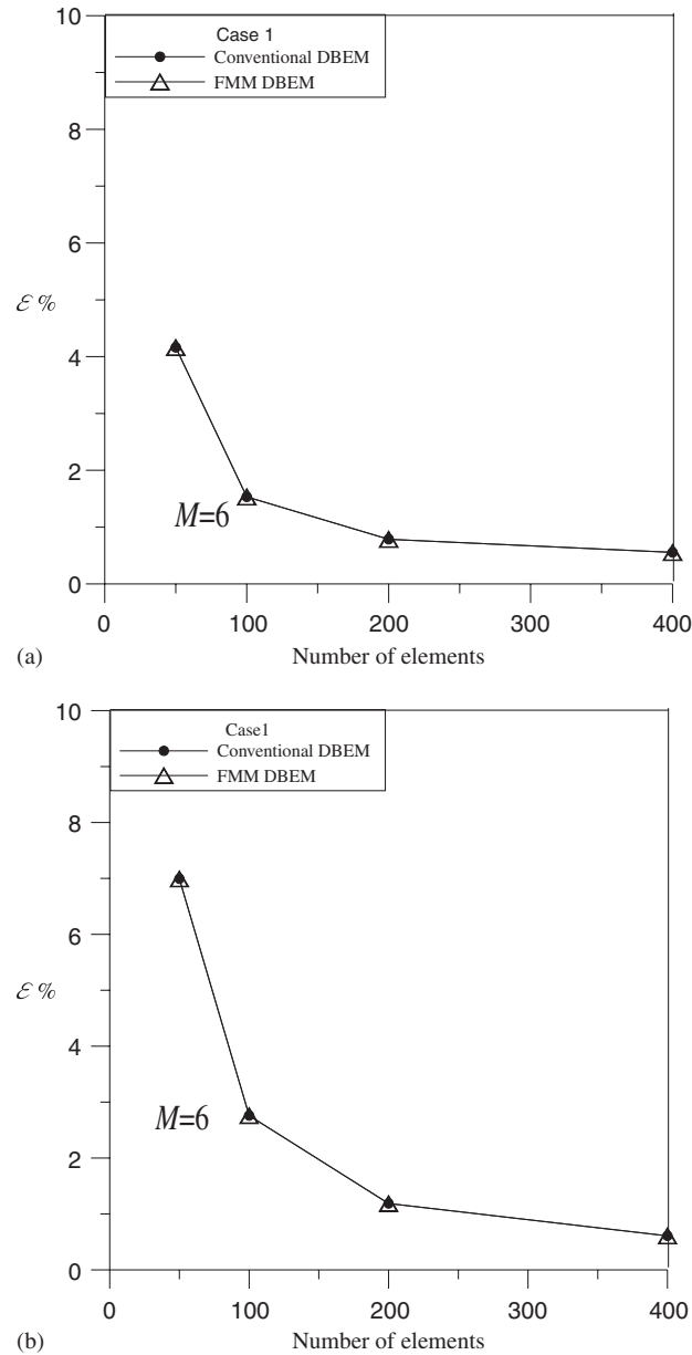
Figure 5. The relative error, \varepsilon , against the number of boundary elements (a) using the UT method and (b) the LM method for case 1.
